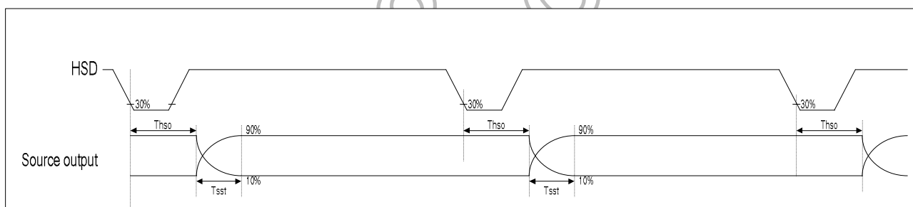
Figure 10. 2 Source Output Timing Diagram
