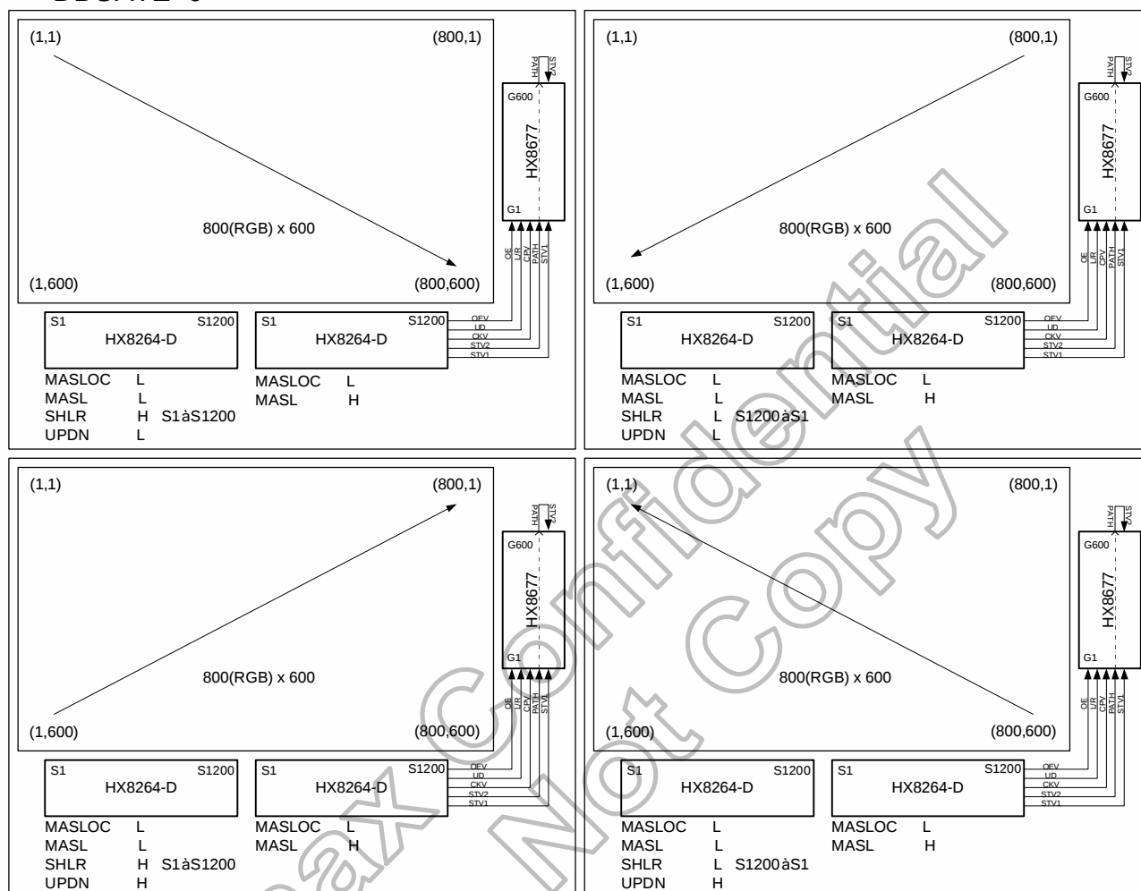
Figure 3. 7 HX8264-D Two Chip Cascade 800(RGB) x 600 Application Block Diagram-2
