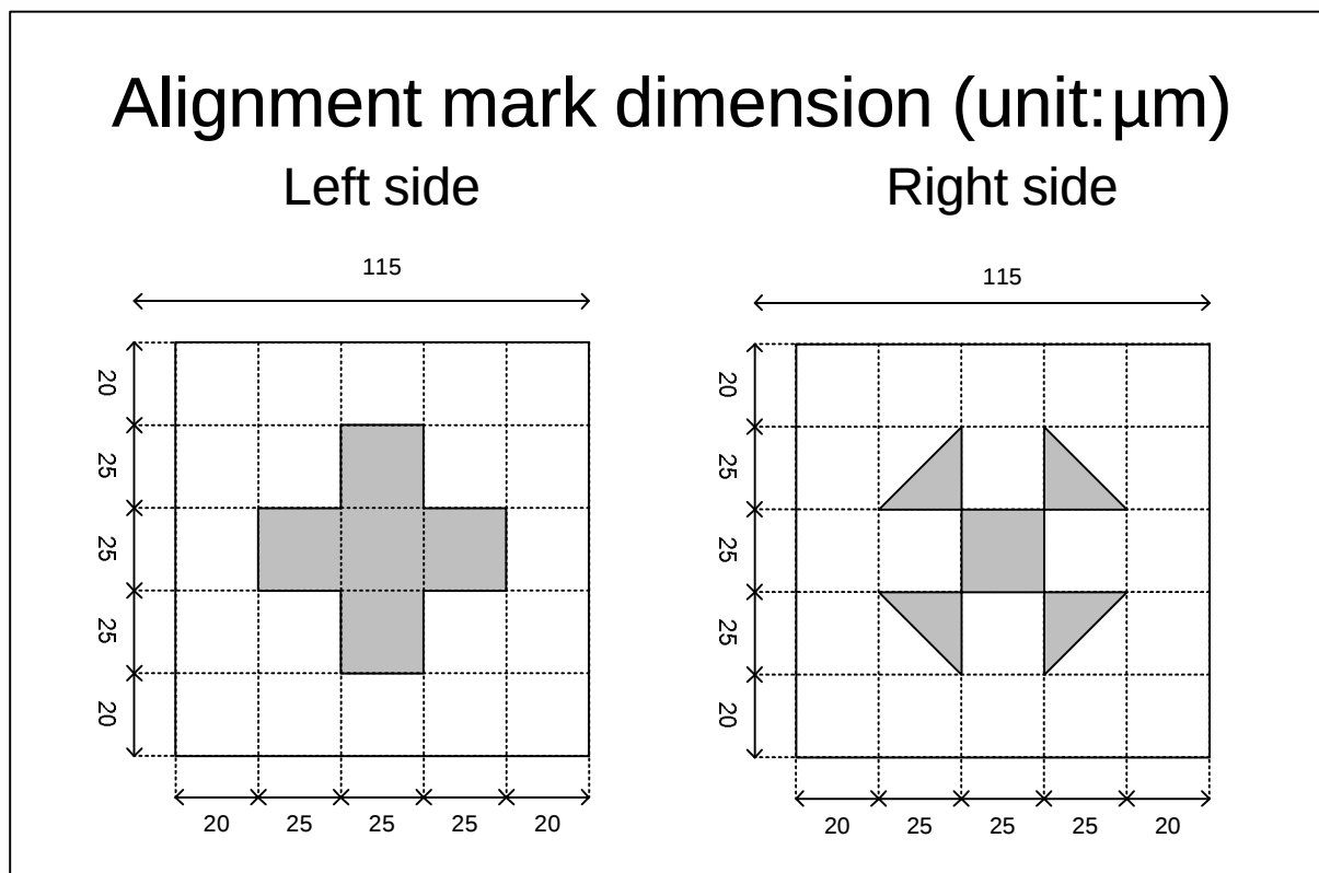
Figure 12. 2 Alignment Mark
