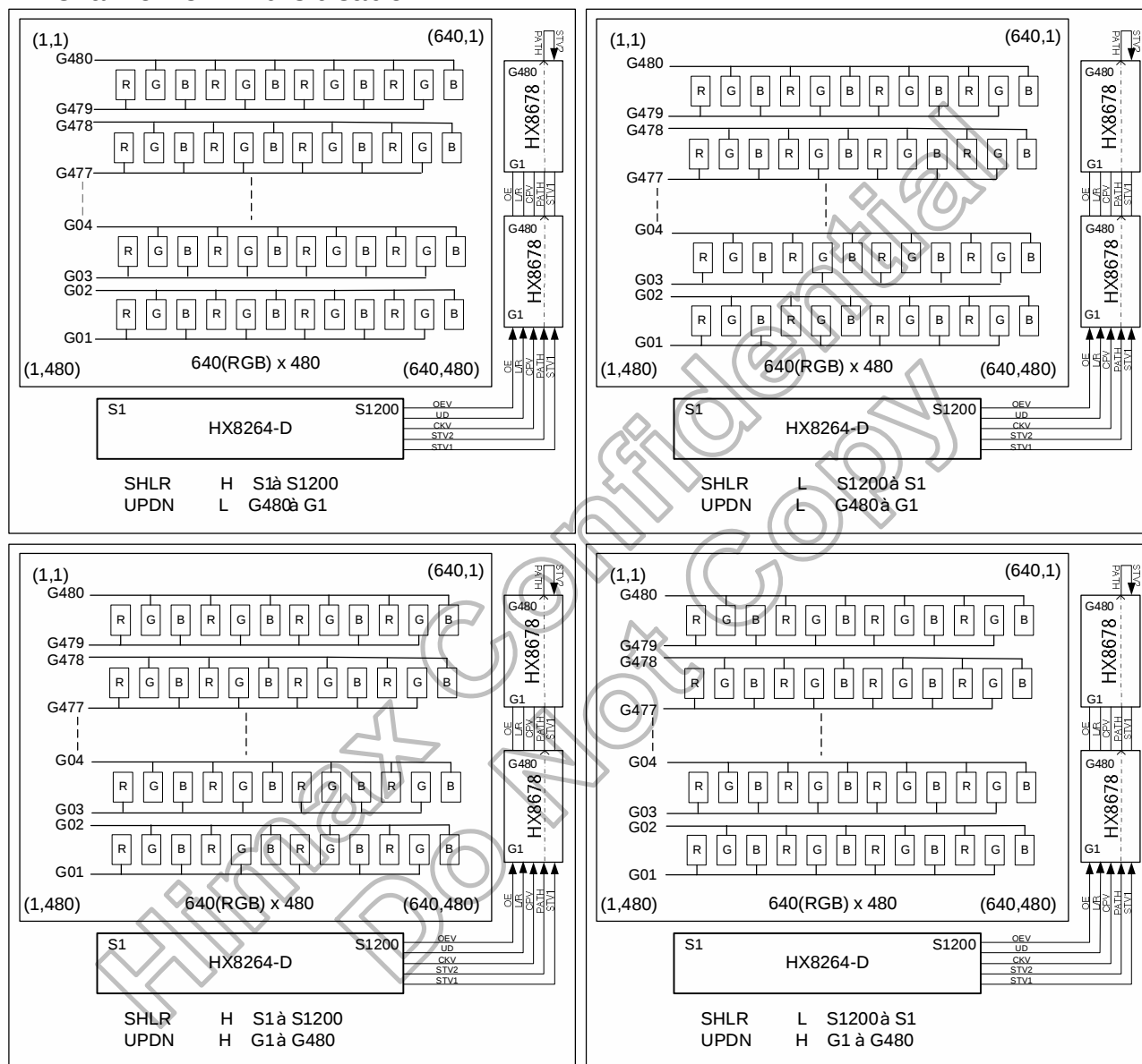
Figure 3. 15 HX8264-D Dual Gate 640(RGB) x 480 Application Block Diagram-2
