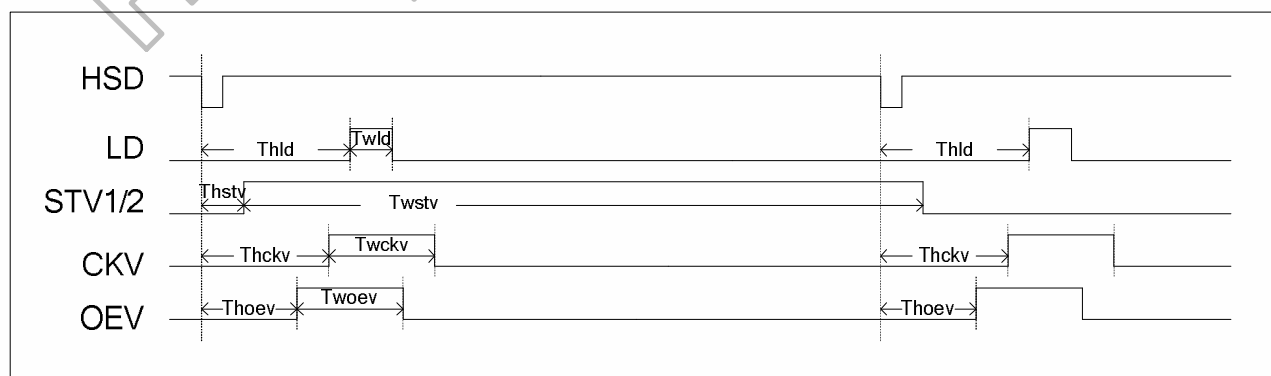
Figure 10. 6 Gate Output Timing Diagram (Cascade)
