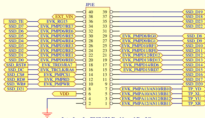
Interface for PIC24/32 Eval board Rev2C
