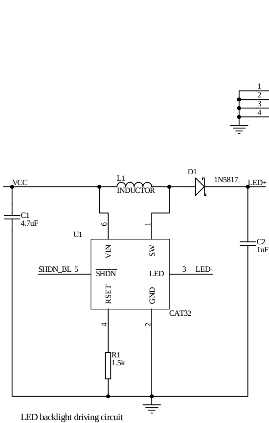
LED backlight driving circuit
